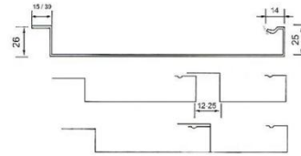
C7 型轻质吸音吊顶灯 Type C7 Light-duty Sound-deadening Furred Ceilings
